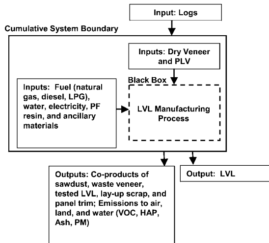
FIG. 2. The cumulative system boundary to define the life-cycle inventory of producing laminated veneer lumber (LVL); environmental burdens are included for production of veneer and parallel laminated veneer (PLV) but exclude those for the logs input to these products.
