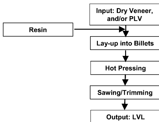
FIG. 1. Process steps for the production of laminated veneer lumber; if green veneer is input, then a drying step is added prior to resin application.
