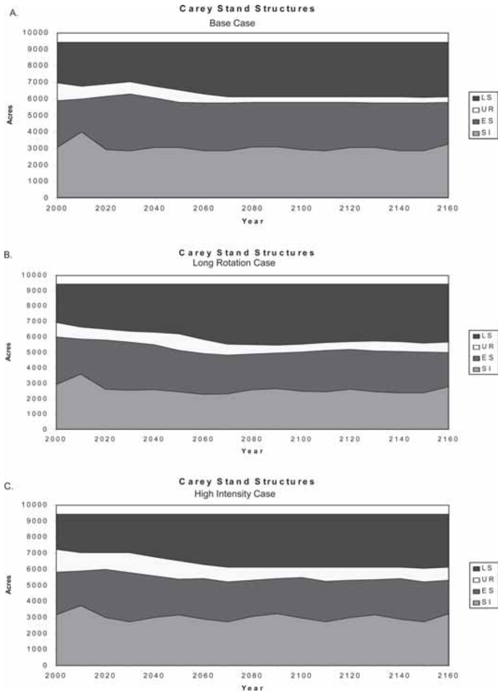
FIG. 2. A. Stand Structures through time for the Base Case. B. Stand Structures through time for the Long Rotation Case. C. Stand Structures through time for the High Intensity Case. LS – Late Seral; UR – Understory Reinitiation; ES – Exclusion Structure; SI – Stand Initiation.
