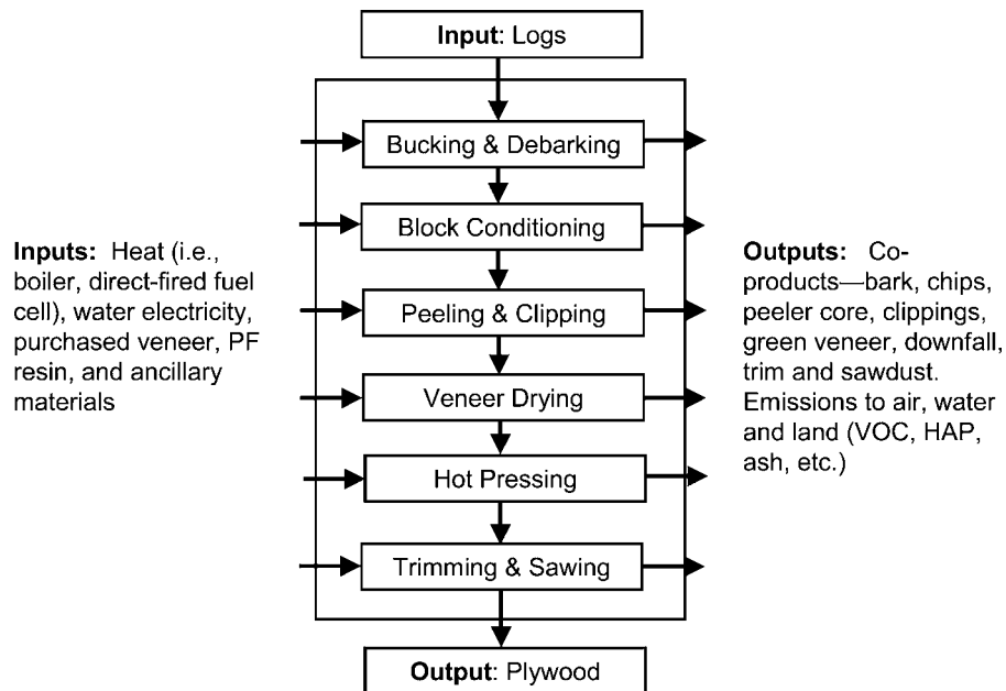
FIG. 1. Unit process approach to the modeling of the plywood manufacturing process.
