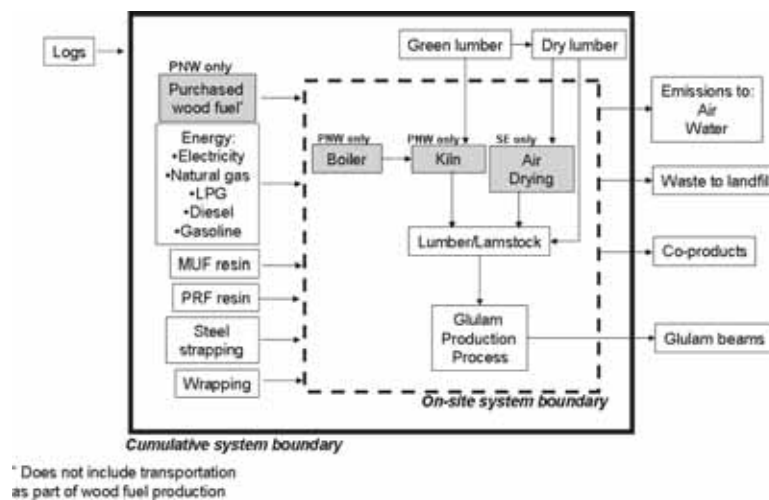
FIG. 2. Cumulative (solid line) and on-site (dotted line) system boundaries for glulam production used to model the PNW and SE manufacturing process. Burdens associated with electricity and fuel production, resin and lumber production, raw material production, and transportation are not included within the on-site system boundary. Forest growth, management, and harvesting, wood fuel production, and transportation are not included in the cumulative system boundary.
