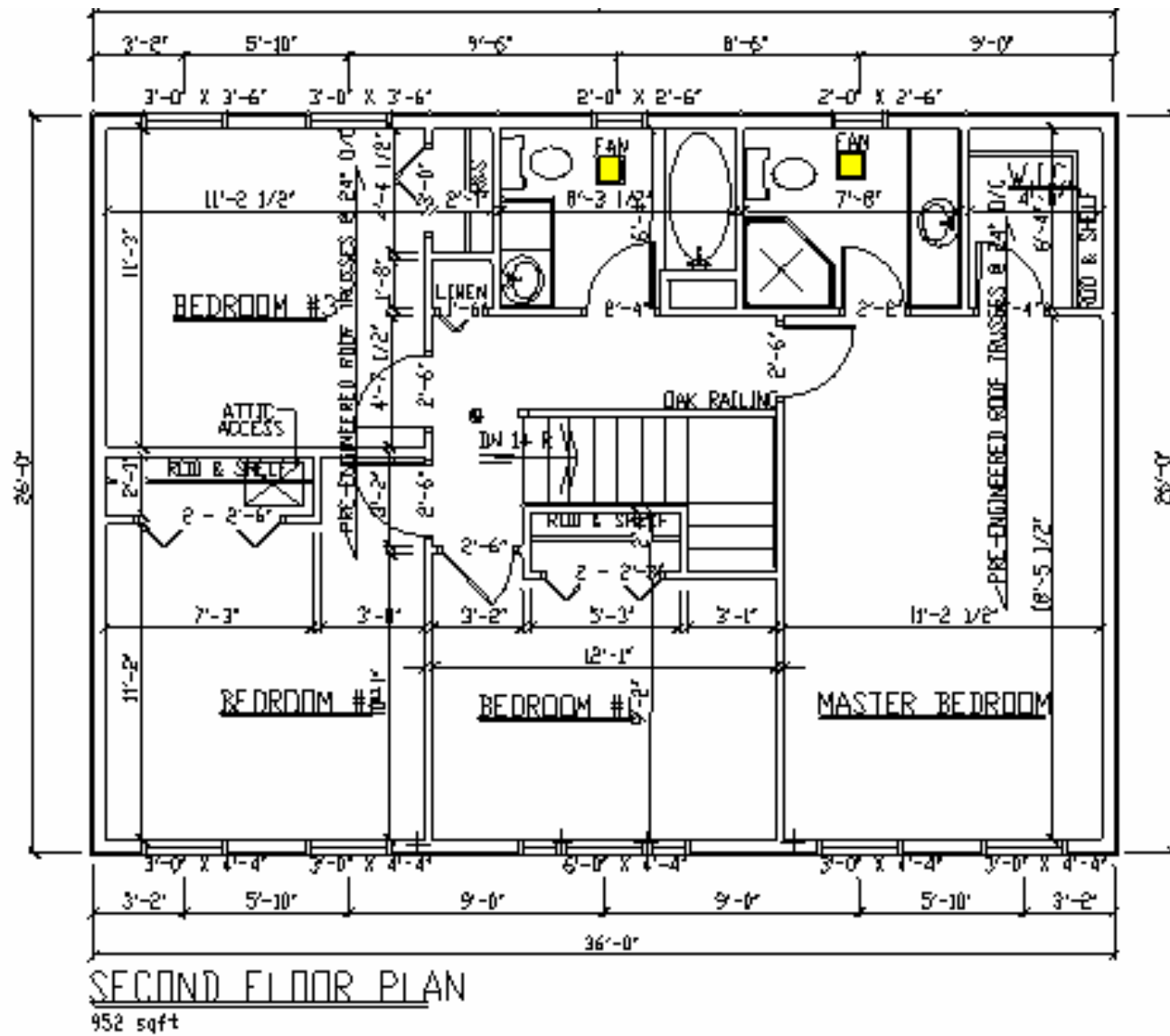
Figure B 11. Minneapolis house - 2nd floor framing plan and wall topology.
