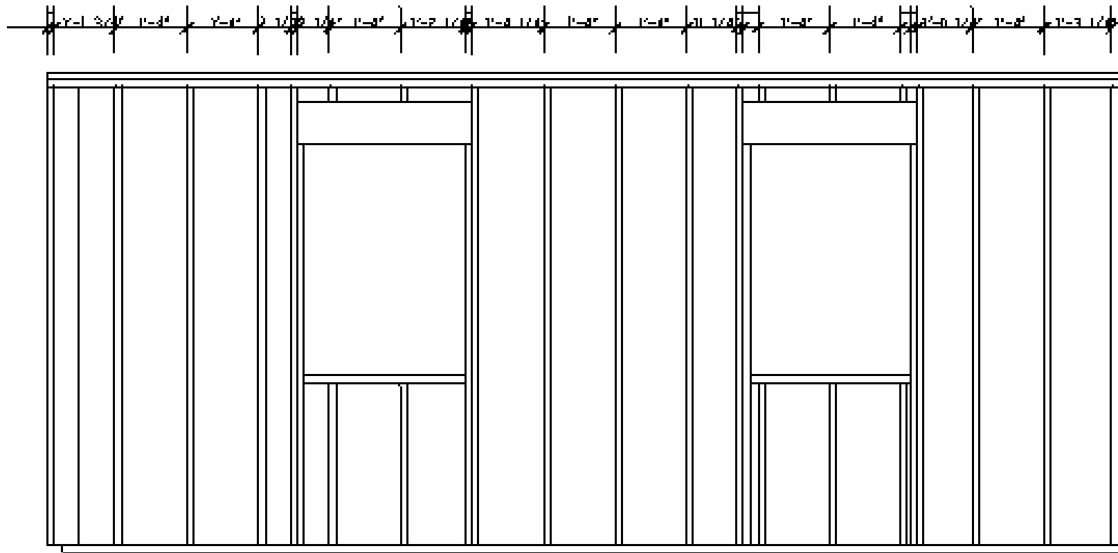
FIGURE B.6. Minneapolis house - typical wall framing.
