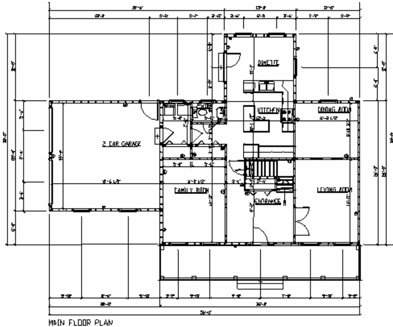
Figure B 3. Minneapolis house - main floor plan.
