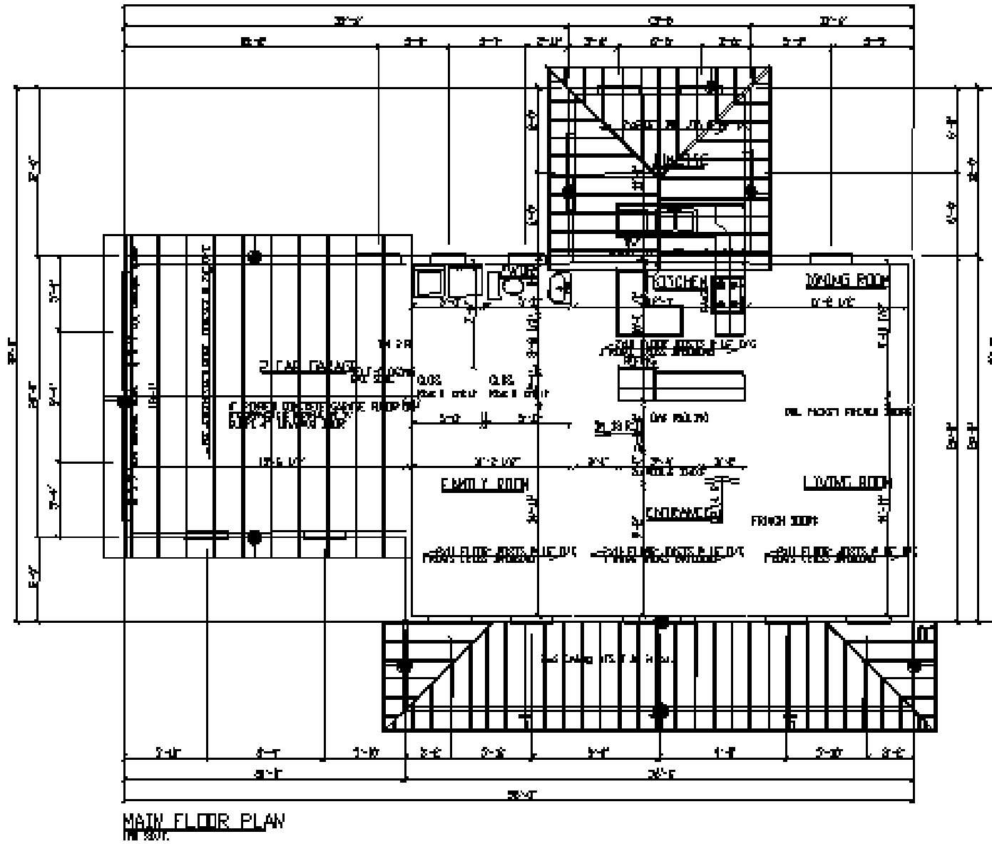
Figure B 9. Minneapolis house - main floor plan with roof and floor framing.
