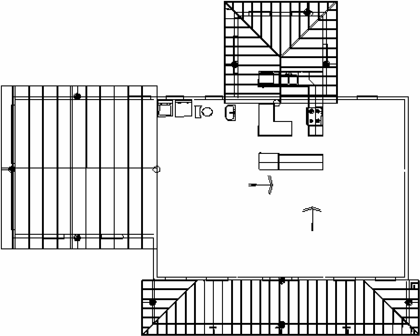
Figure B 8. Minneapolis house - main floor plan with roof and floor framing.
