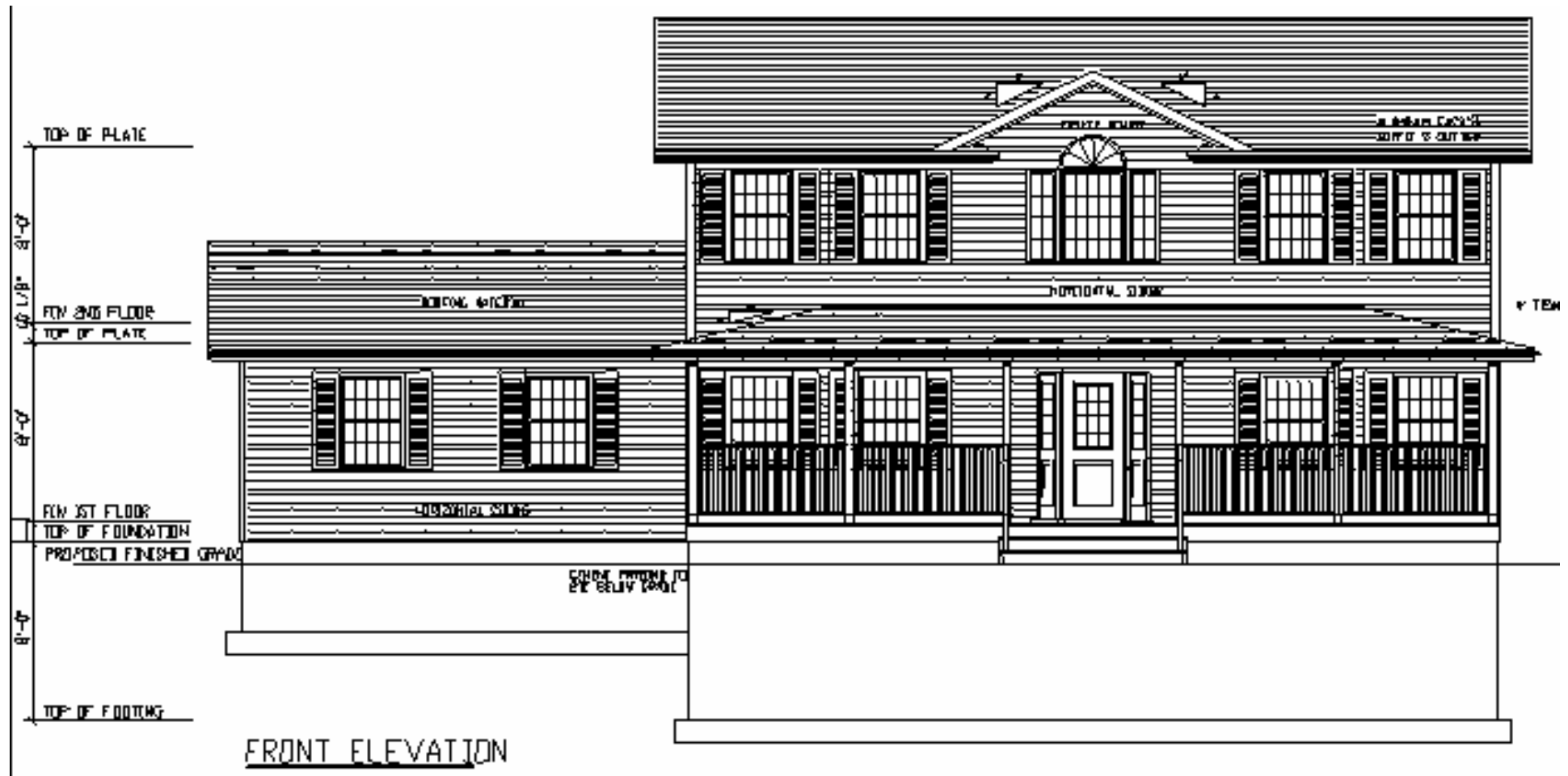
Figure B 14. Minneapolis house - front elevation.
