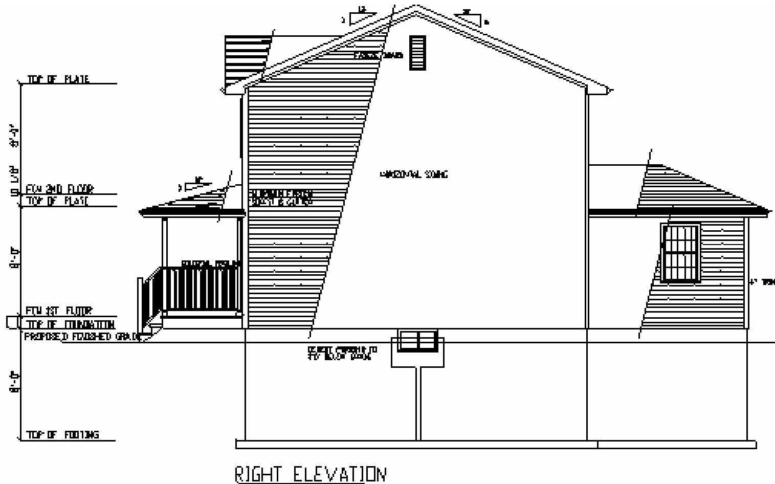
Figure B 17. Minneapolis house - right elevation.
