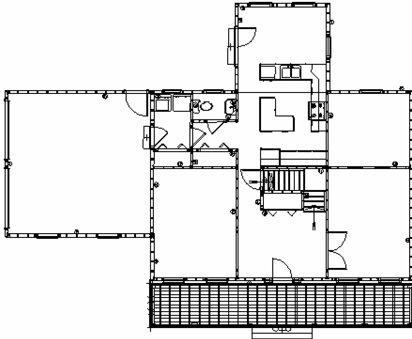
Figure B 4. Minneapolis house - main floor plan.
