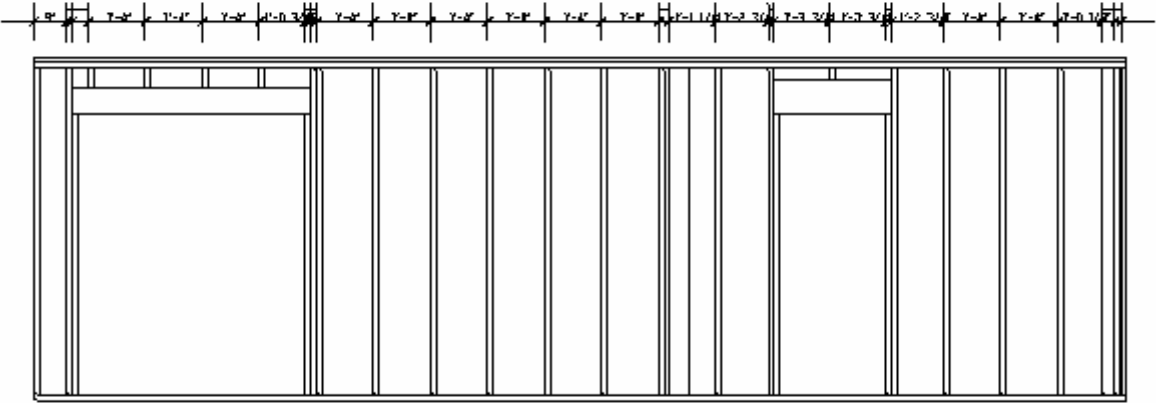
2x4 WALL NO. 16
